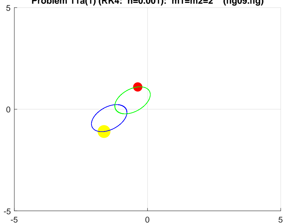
Celestial Mechanics: Two (2) Body Problem Problem 11a(1) (RK4: h=0.001 ): m_1=m_2=2 (fig09.fig)
